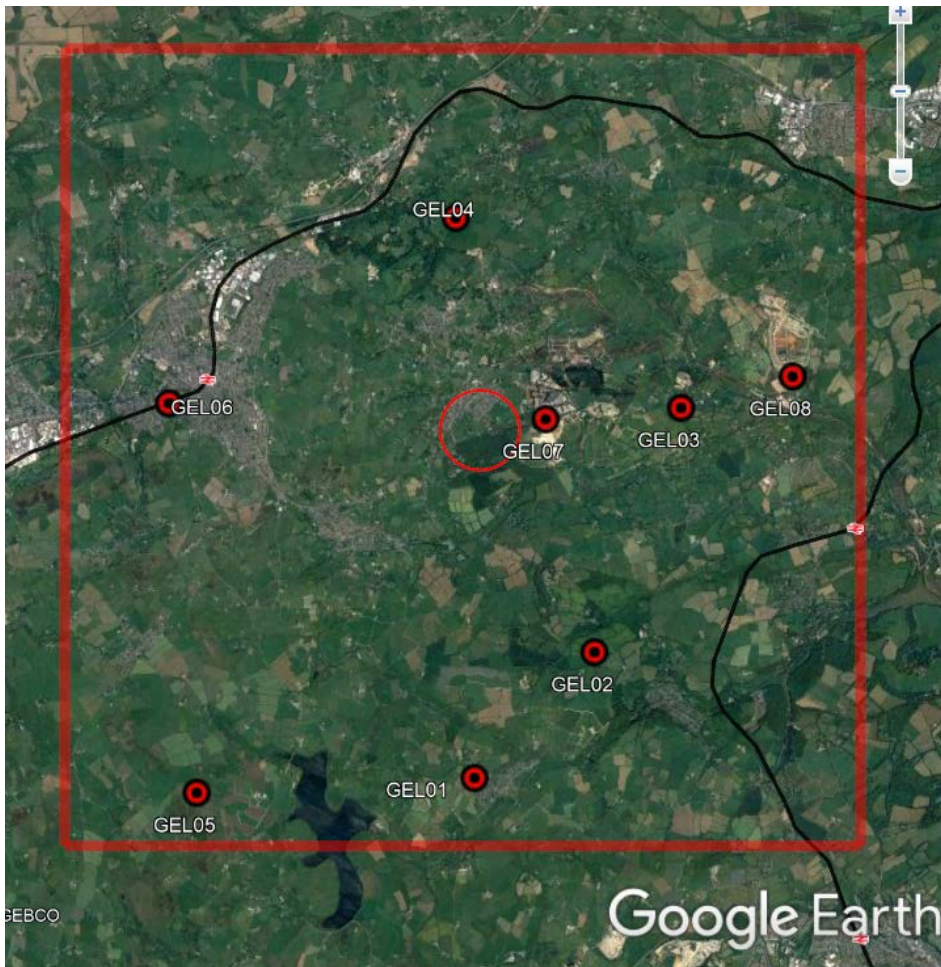
Figure 4: Aerial photograph showing the layout of the eight microseismic stations, where GEL07 is the borehole sensor on the UDDGP drill site. The red 500m radius circle indicates the approximate location of the subsurface target and the red square the 10km x 10km overall monitoring area.
