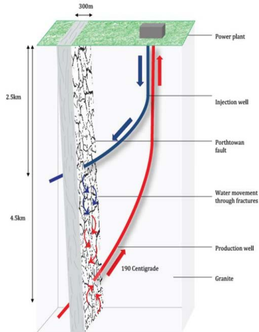
Figure 2: Cartoon of the UDDGP concept showing idealized well intersections with the PTF
