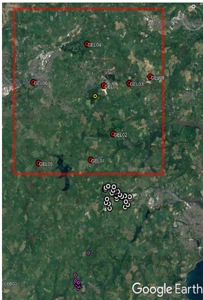
Figure 6: Aerial photograph showing the location of the UDDGP associated seismicity (yellow points), where GEL07 is the borehole sensor on the UDDGP drill site. The red square is the 10km x 10km overall monitoring area. Also shown are the quarrying related blasts (white points) and the Constantine swarm (purple points).
