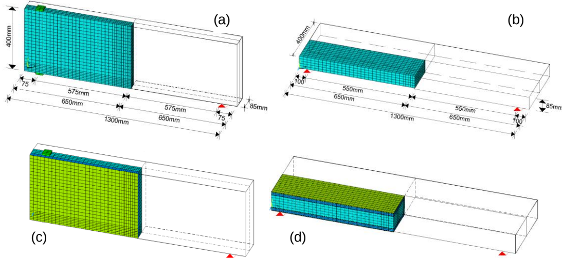
Figure 12. Schematic arrangement and geometry of control specimens: (a) in-plane model, Series B ("beam-columns"), (b) out-of-plane model, Series D-"s". View of model for (c) Specimen 1iMi1 for in-plane loading and (d) Specimen 2iMi2 for out-of-plane loading.
