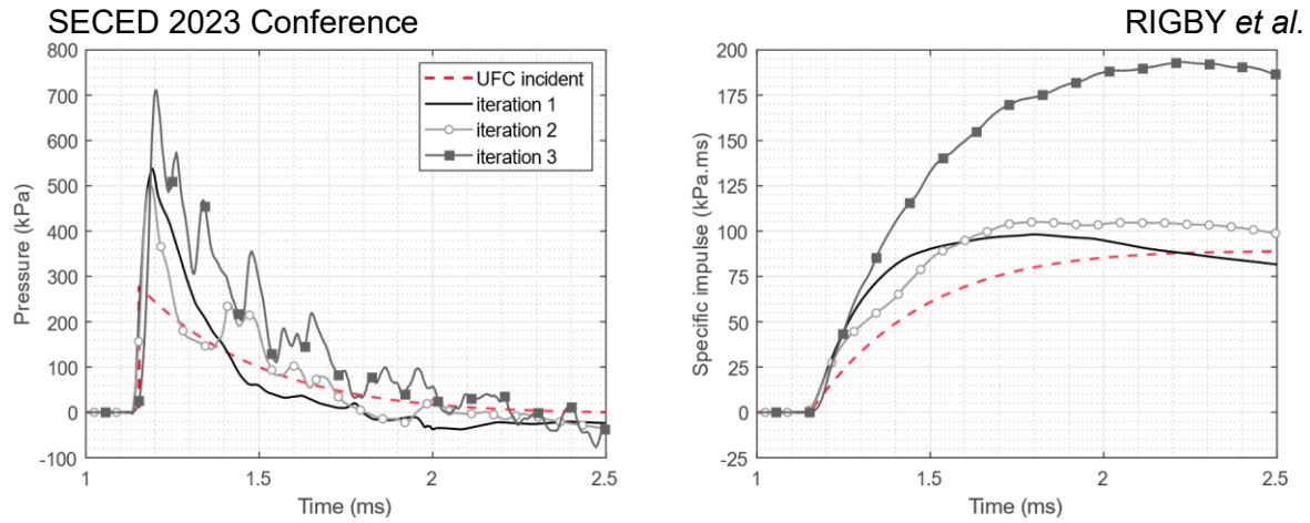
Figure 7. “On-obstacle” reflected pressure and specific impulse histories (S12; 1.35 m slant distance from a 250 g PE4 hemisphere). UFC incident predictions shown in red.
