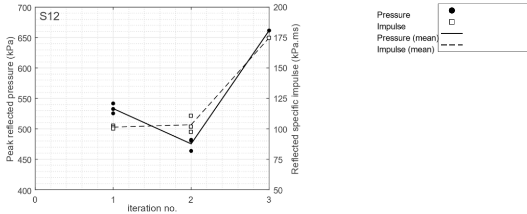
Figure 8. Compiled peak pressure and peak specific impulse [secondary y-axis] with increasing pre-fractal iteration for S4, S11, and S12 (250 g hemisphere at 1.25 m stand-off from the front-face of the central obstacle)
