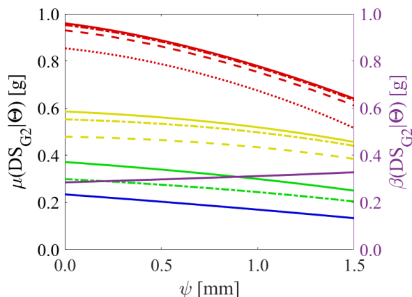
Figure 6. Evolution of the fragility median values and dispersion as a function of \psi .
