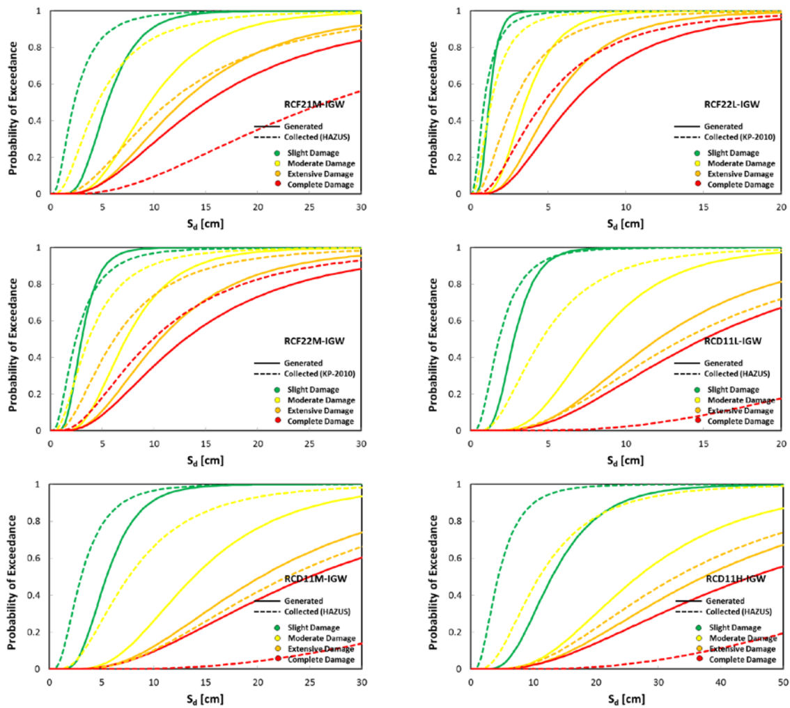
Figure 3. Comparison between the generated (customized) fragility curves and the collected (existing, assigned) fragility curves as provided by HAZUS-MH (FEMA 2003) and KP2010 (Kappos and Panagopoulos 2010).
