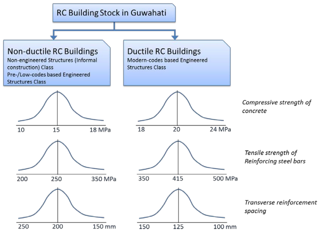
Figure 2. Range of expected values of the structural characteristics-related parameters for the existing RC buildings in Guwahati
